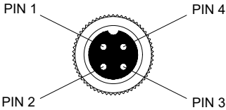
4 PIN FEMALE MATING FACE
