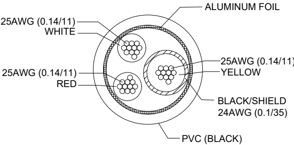
CABLE BUILDUP
